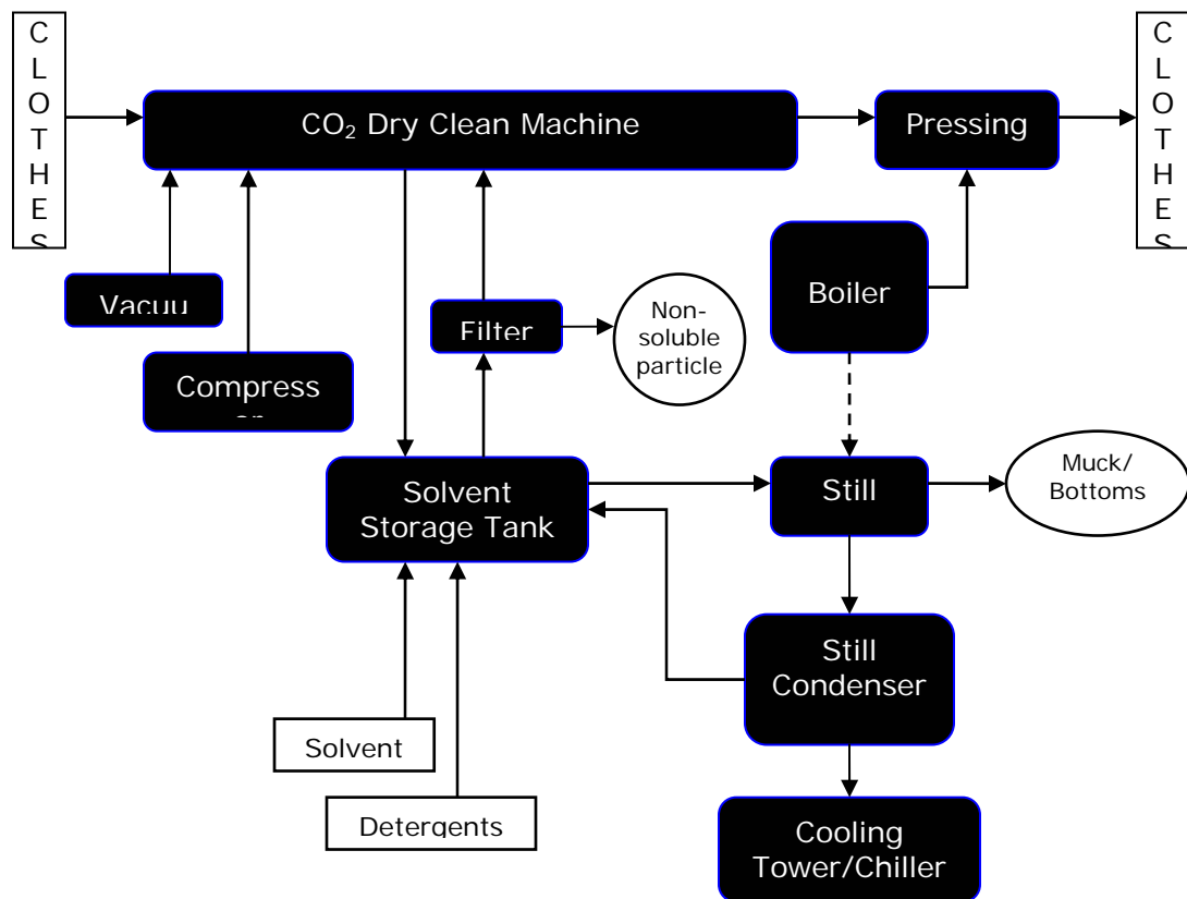
FIGURE 2. ENERGY PROCESS FLOW DIAGRAM FOR CO 2 DRY CLEAN MACHINE 19
