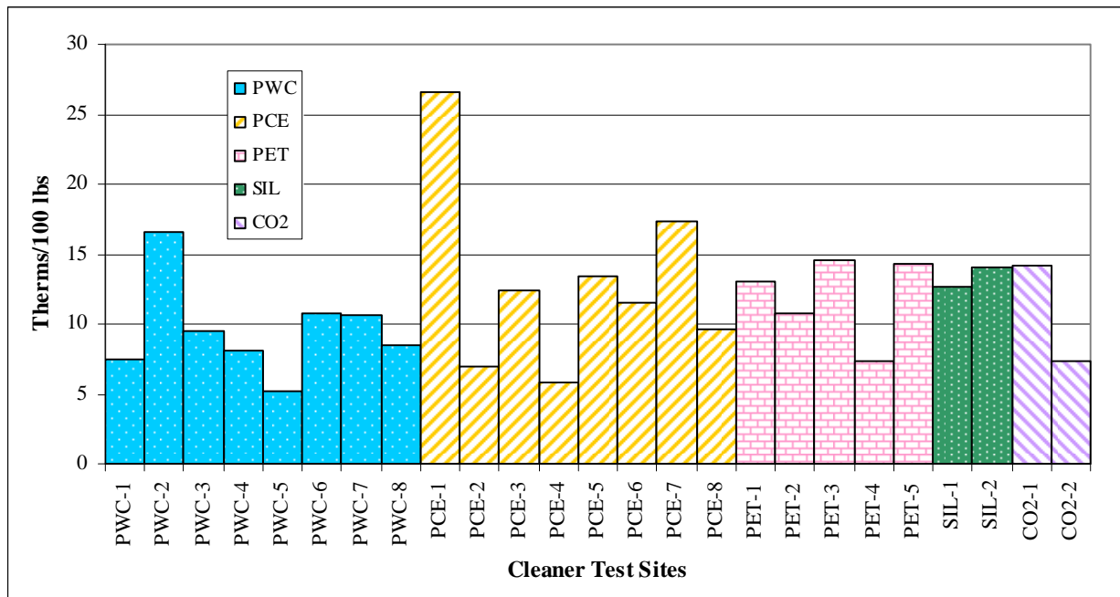
FIGURE 8. NATURAL GAS USE FOR FIVE GARMENT CARE TECHNOLOGIES STANDARDIZED PER 100 POUNDS CLEANED
