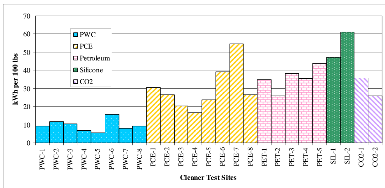
FIGURE 4. ELECTRICITY USE FOR FIVE GARMENT CARE TECHNOLOGIES
