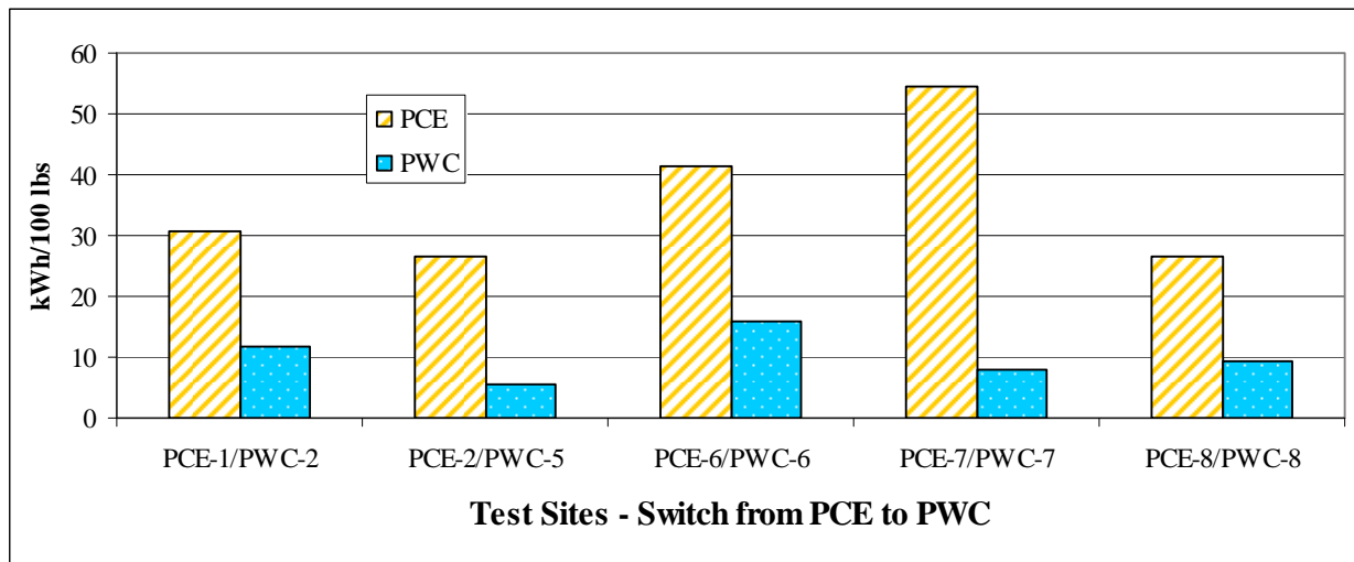
FIGURE 5. COMPARISON OF ELECTRICITY USE AT TEST SITES SWITCHING FROM PCE DRY CLEANING TO PWC, STANDARDIZED PER 100 LBS CLEANED
