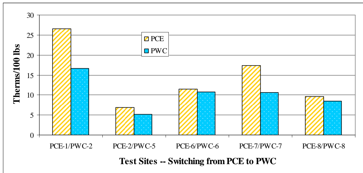
FIGURE 9. COMPARISON OF NATURAL GAS USE AT TEST SITES SWITCHING FROM PCE DRY CLEANING TO PWC, STANDARDIZED PER 100 POUNDS CLEANED
