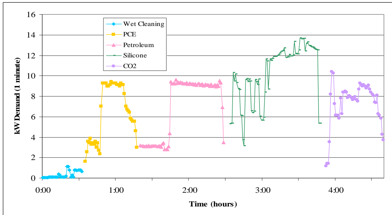
FIGURE 6. ONE-MINUTE kW DEMAND DURING WASH AND DRY CYCLE FOR FIVE GARMENT CARE TECHNOLOGIES 34
