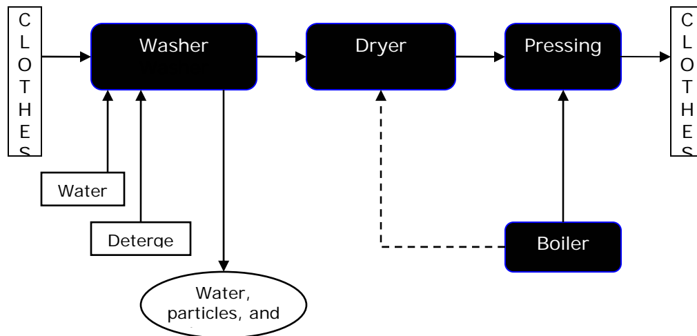
FIGURE 3. PROCESS FLOW DIAGRAM FOR PROFESSIONAL WET CLEAN SYSTEM 21
