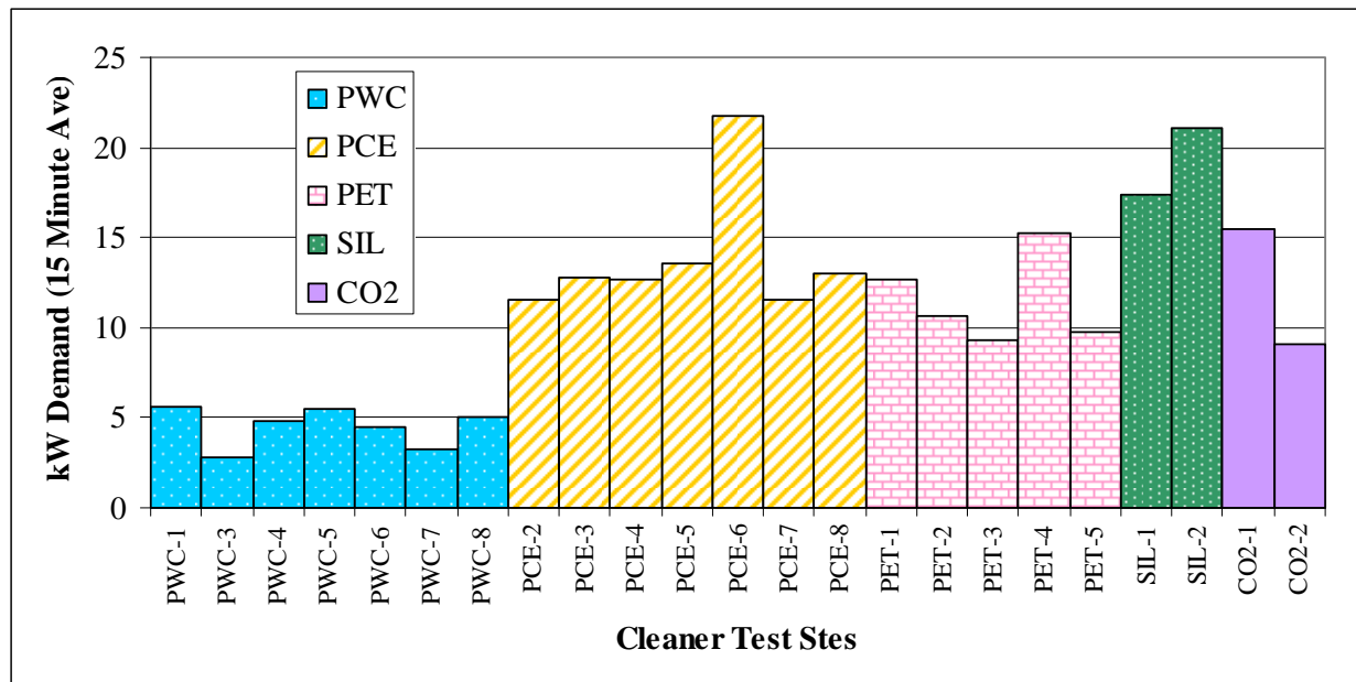
FIGURE 7. 15-MINUTE PEAK kW DEMAND FOR FIVE GARMENT CARE TECHNOLOGIES
